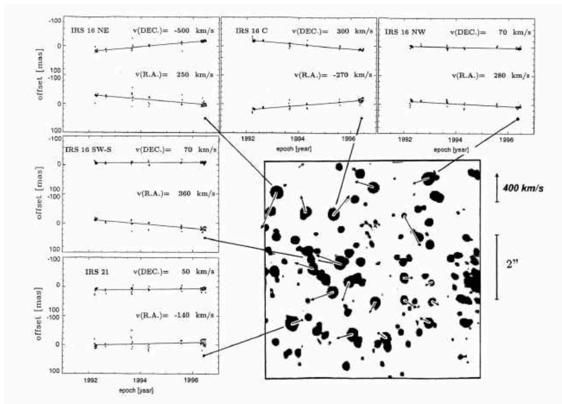
Figure 5. Proper motions and vectors of selected stars surrounding the central compact radio source Sgr A*, marked with a cross. The measurements were carried out over four years and the offsets were determined with respect to the base epoch in 1994. From Eckart & Genzel (1997).
