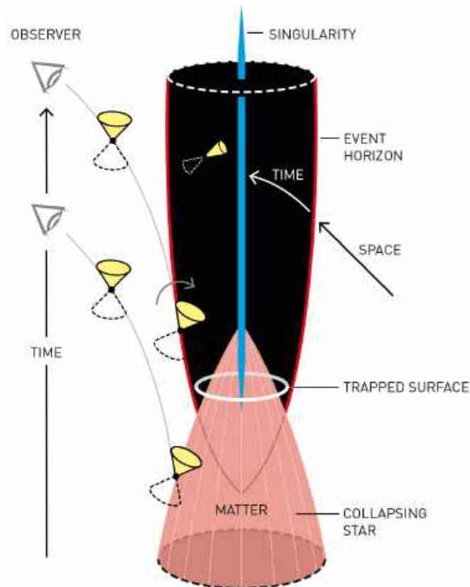
Figure 2. The diagram is based on Penrose's paper from 1965 and shows the collapse of matter into a black hole. On a trapped surface all light cones are tipped inwards, and the formation of a singularity is inevitable.
