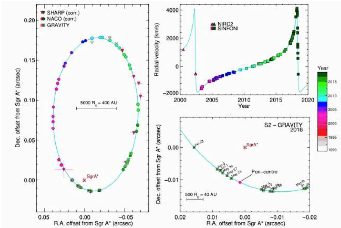
Figure 9. Summary of the observational results of monitoring the S2–Sgr A* orbit from 1992 to 2018. Left: Projected orbit of the star S2 on the sky (J2000) relative to the position of the compact radio source Sgr A* (brown crossed square at the origin). Triangles and circles (and 1\sigma uncertainties) denote the position measurements with SHARP at the NIT and NACO at the VLT, color-coded for time (colour bar on the right side). The cyan curve shows the best-fitting S2 orbit to all these data, including the effects of general and special relativity. The bottom right panel shows a zoom-in around pericentre in 2018. Upper right: Radial velocity of S2 as a function of time (squares: SINFONI/NACO at the VLT; triangles: NIRC2 at Keck). S2 reached pericentre of its orbit at the end of April 2002, and then again on 19 May 2018. The cyan curve shows the best-fitting S2 orbit to all these data, including the effects of General and Special Relativity. From Abuter et al. (2018).
